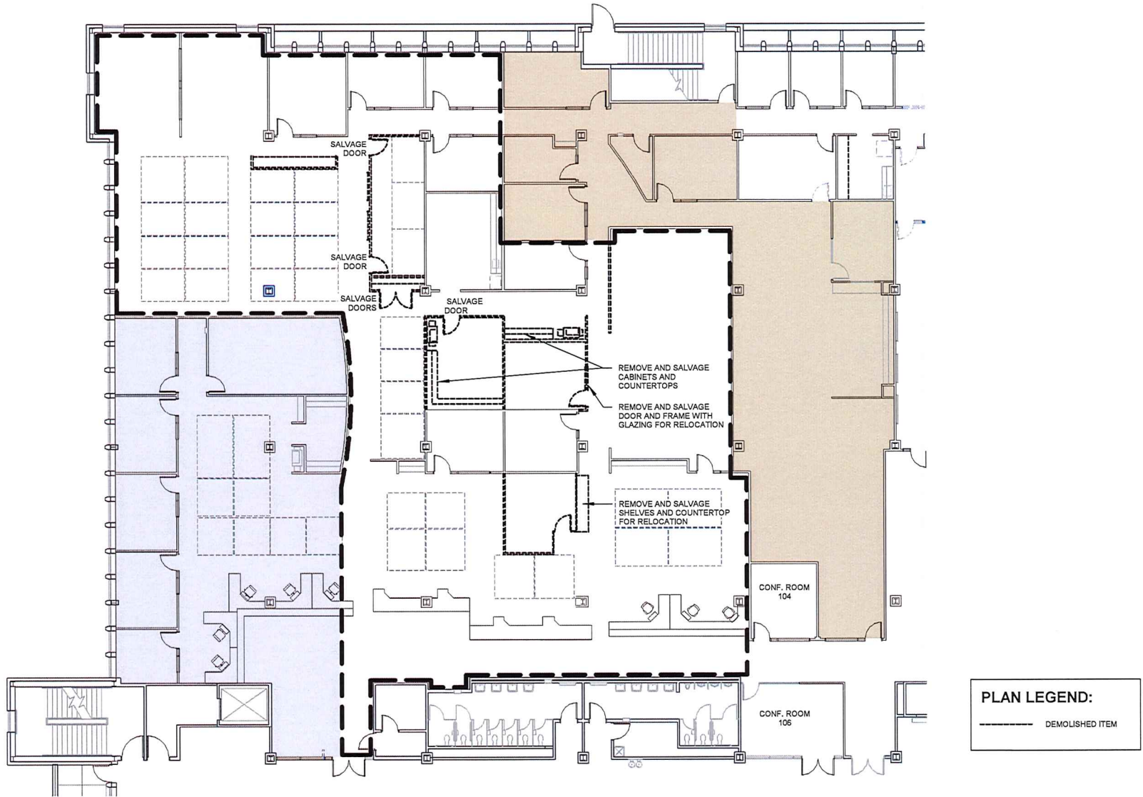
2 DEMOLITION FLOOR PLAN - LEVEL 1
