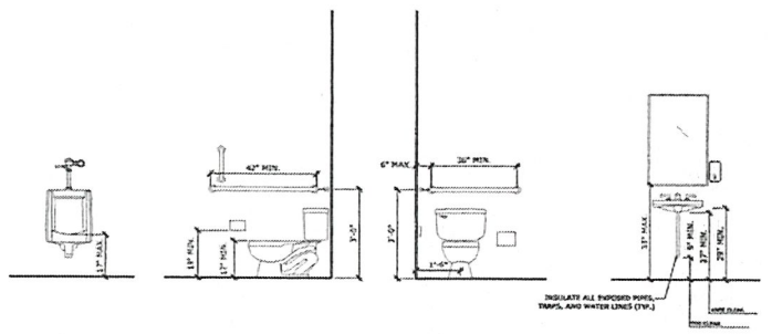
C1 TYP RESTROOM DETAILS A2.03 SCALE: 1/2" = 1'-0"
