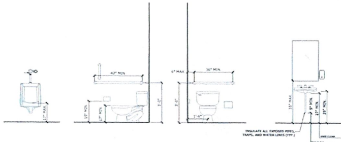
TYP RESTROOM DETAILS SCALE: 1/2" = 1'-0"
