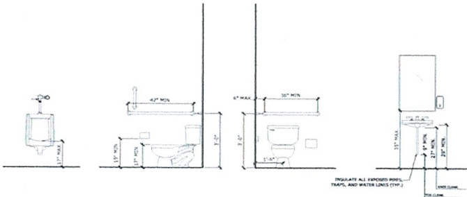
C1 TYP RESTROOM DETAILS A2.01 SCALE: 1/2"=1'-0"
