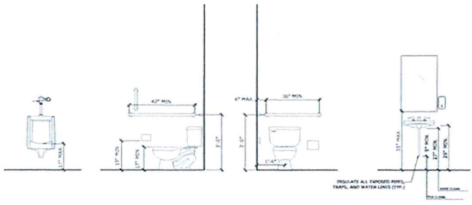
TYP RESTROOM DETAILS SCALE: 1/2"=1'-0"
