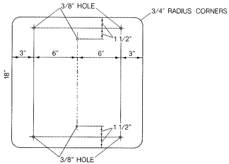
DUAL SIGN MOUNTING PLATE
