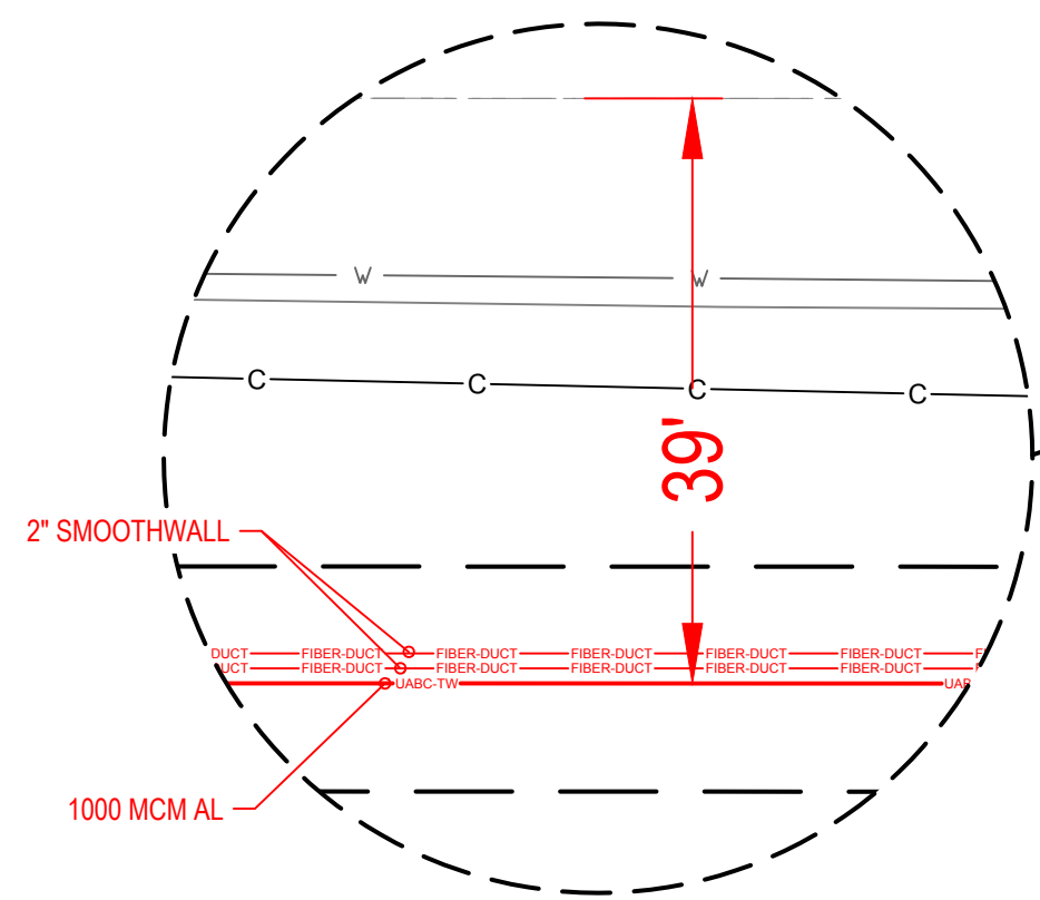
DIRECT BURY FEEDER AND (2) 2" SMOOTHWALLS FOR FUTURE COMMUNICATION IN THE SAME 8" TRENCH NO SCALE
