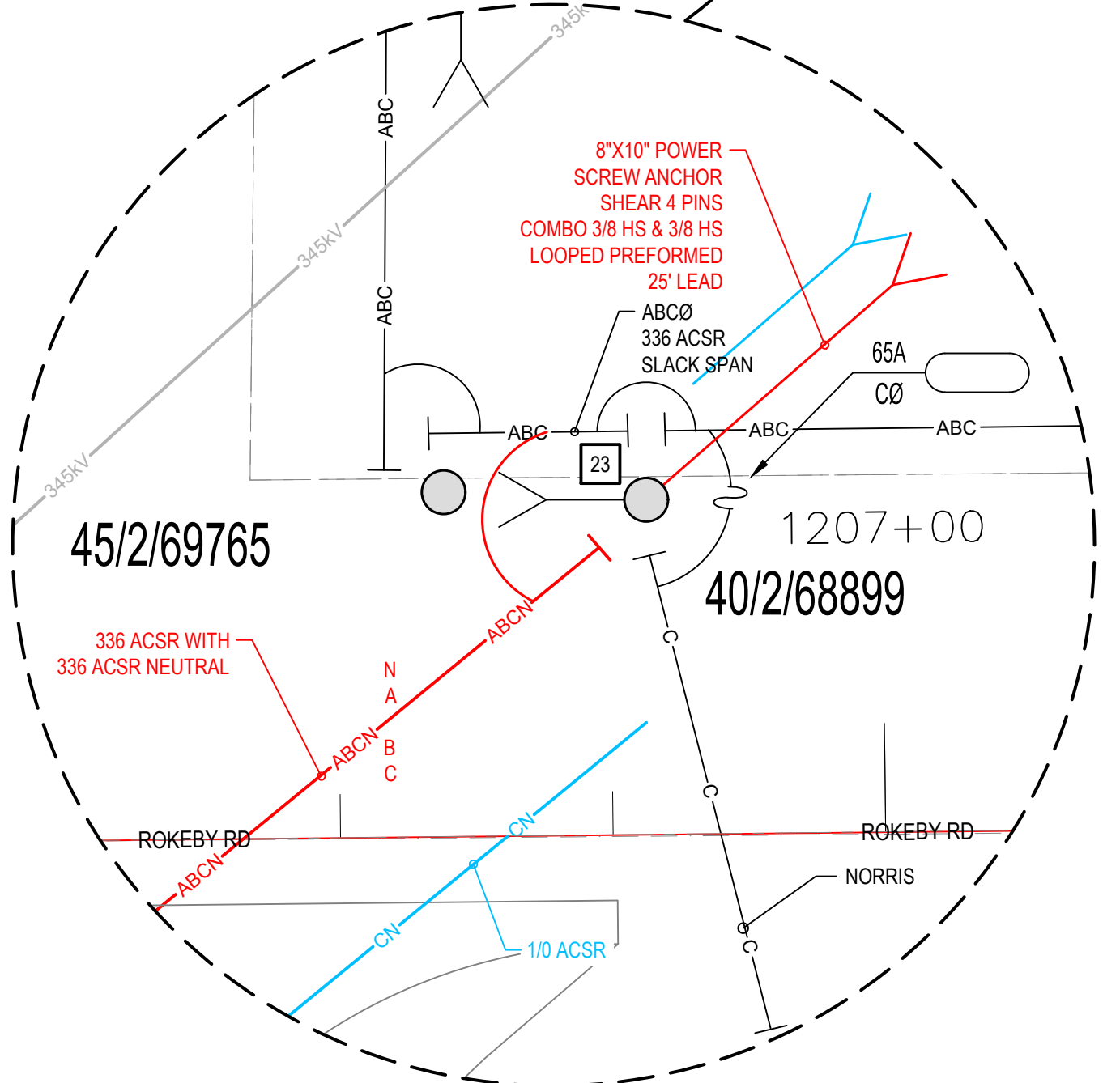
POSITION 23 DETAIL NO SCALE
