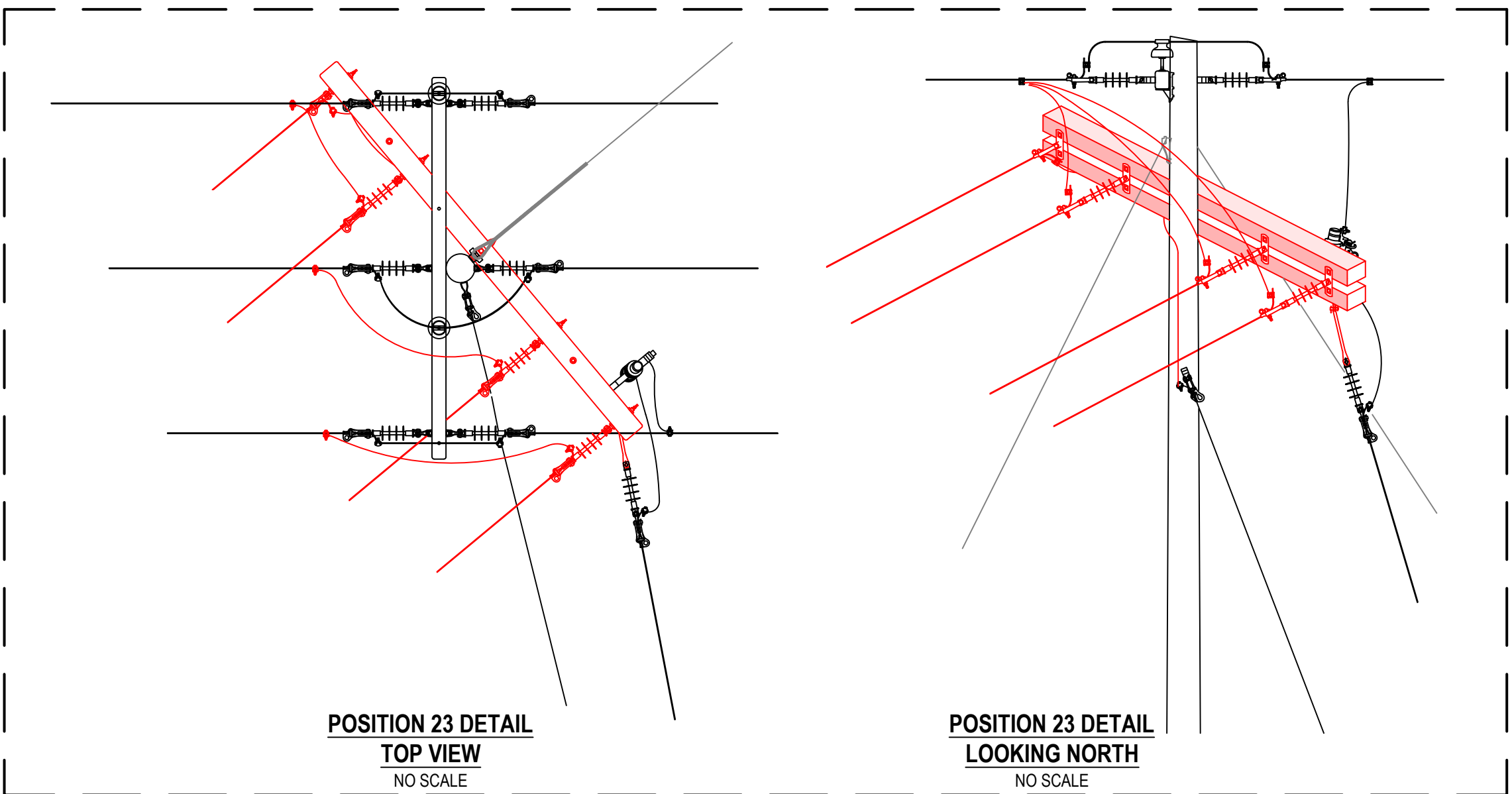
POSITION 23 DETAIL NO SCALE
