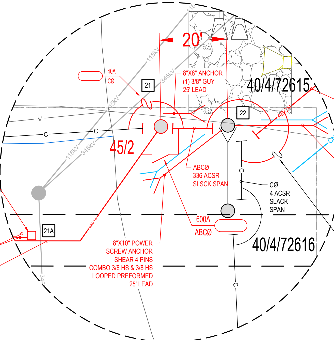
POSITION 21 & 22 DETAIL NO SCALE
