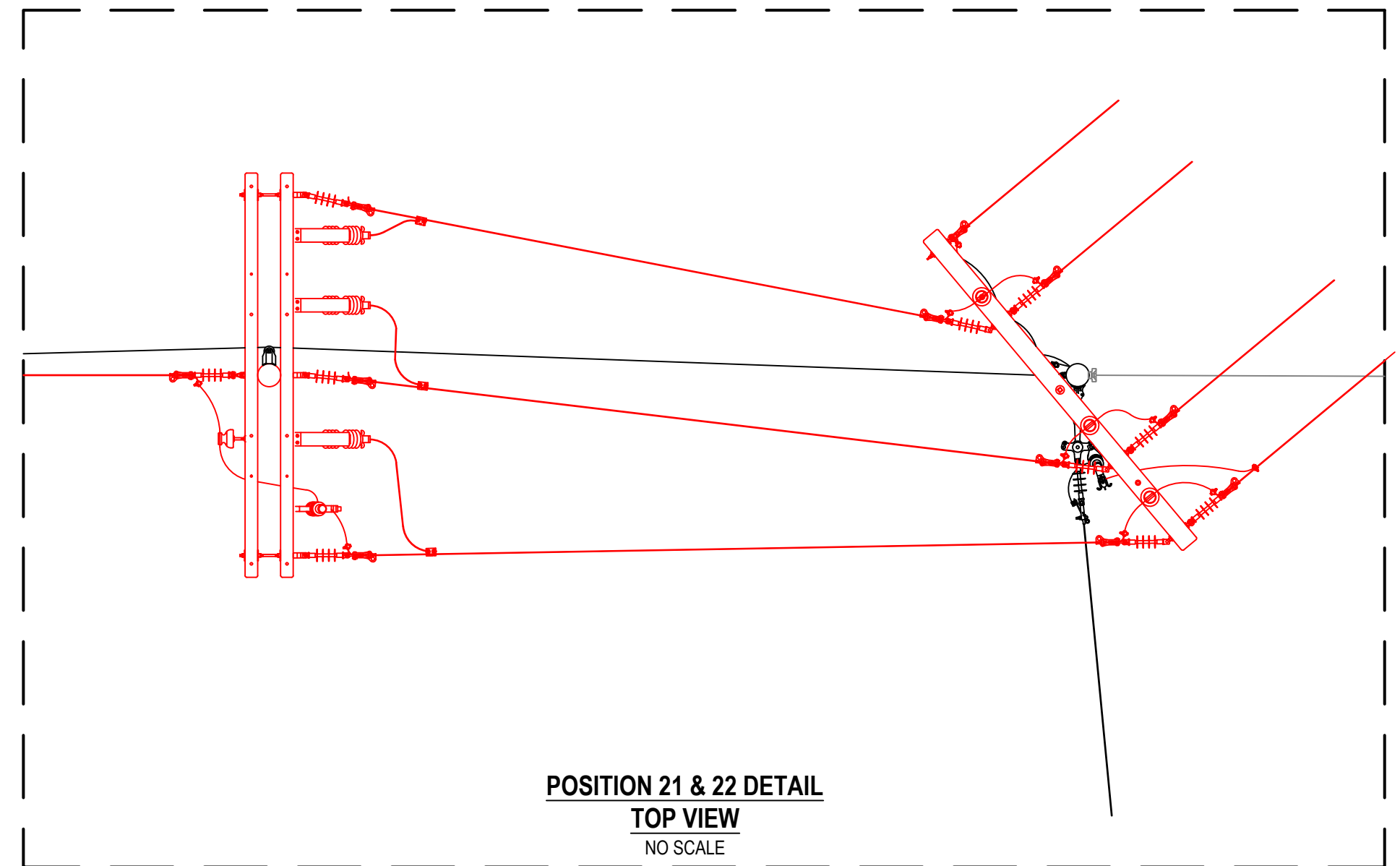
POSITION 21 & 22 DETAIL NO SCALE
